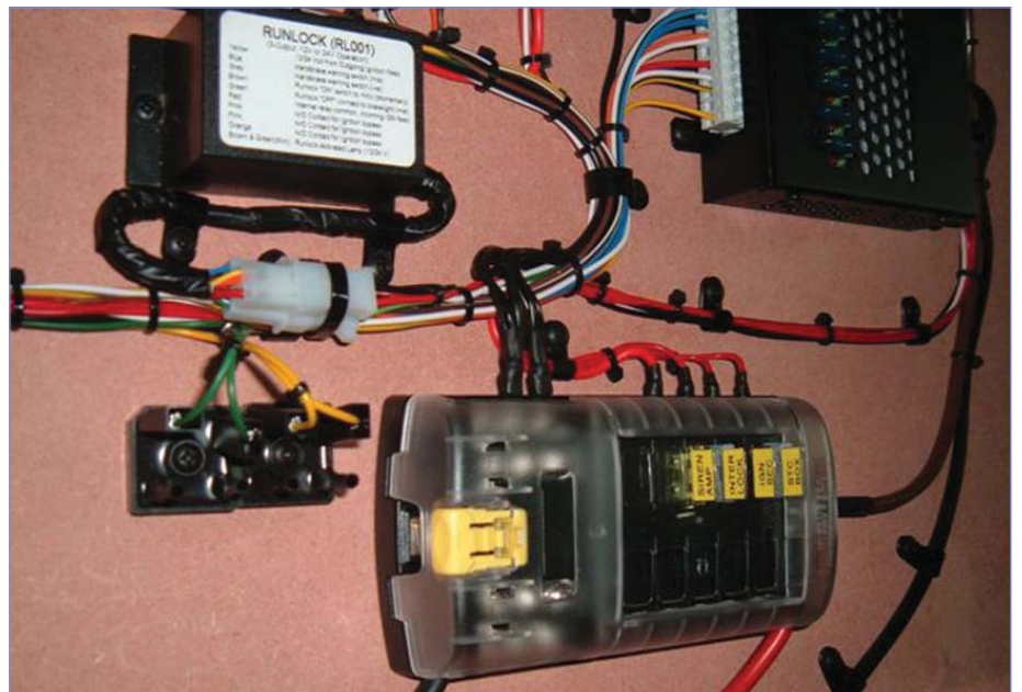
Example of Back Board Layout
